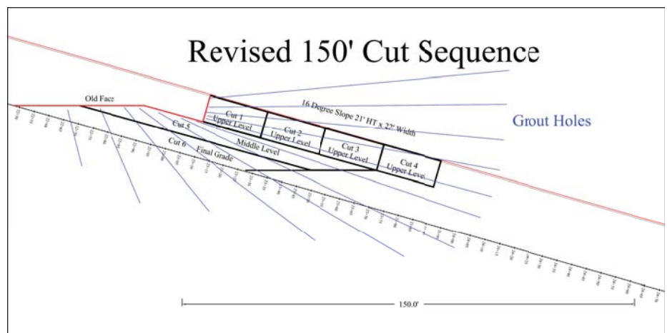
BELOW: Figure demonstrating the general grout hole layout and slope mining sequence for one grout cover. Similar grout cover layout geometry was utilized for treating both primary and secondary permeability, however, more grout holes were required per cover when treating primary permeability.
