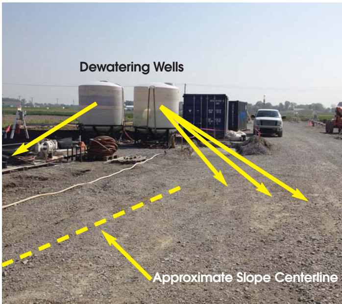
Surface area over slope zone, which encountered the Mt. Carmel Formation. Five dewatering wells were placed on each side of the slope. This picture provides a general idea of the area of slope, which had to be treated, and the spacing and location of dewatering wells.
